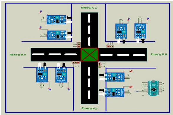
Fig. 2. System design with sensors
