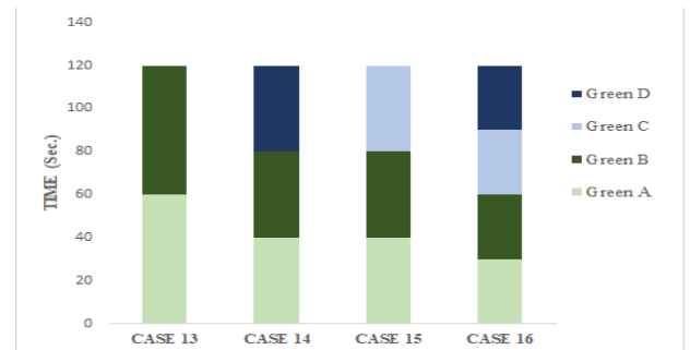
Fig. 10. Group 4 Green signal time
