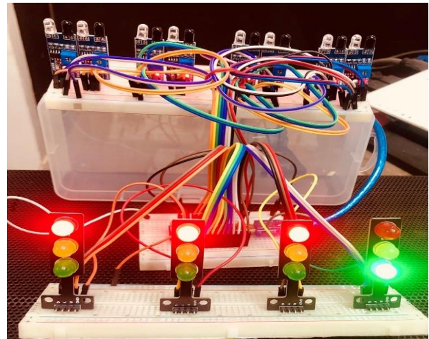
Fig. 4. Prototype Circuit
