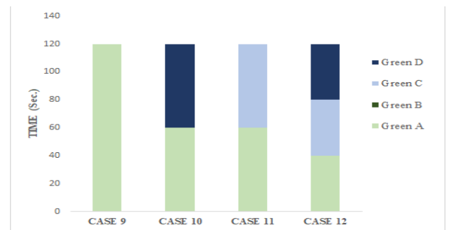
Fig. 9. Group 3 Green signal time
