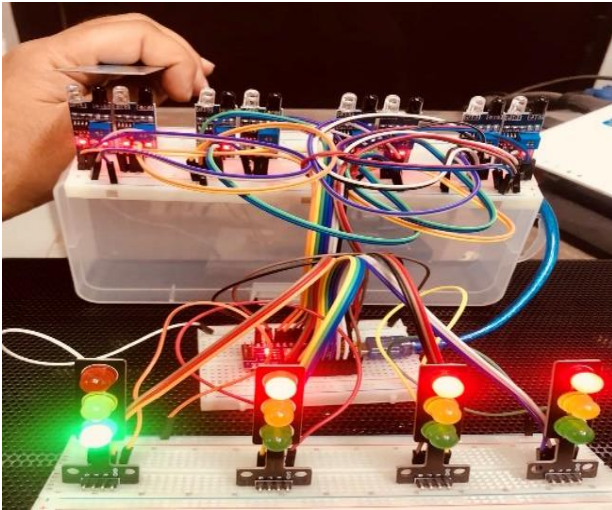
Fig. 5. Prototype Circuit with priority implementation
