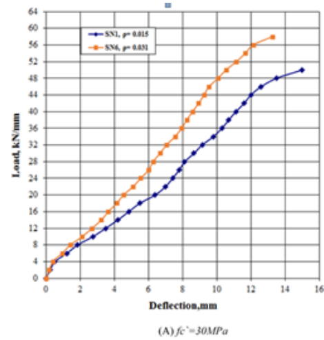
Fig.10. Effect of ( \rho ) for Non-Strengthened Slab Specimens (SN1 and SN6)
