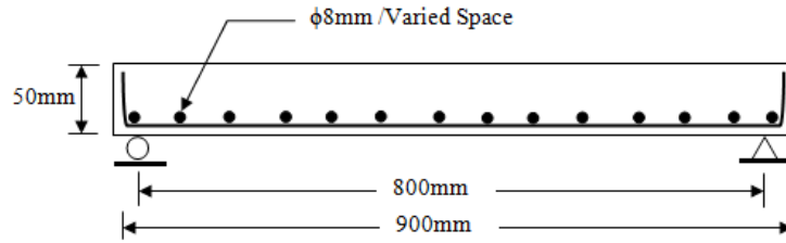
Fig.1. Details of the tested slab specimens
