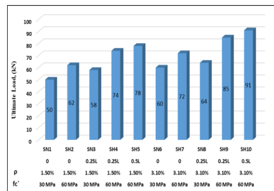
Fig.4. Ultimate Capacity Comparison for all Tested Slab Specimens
