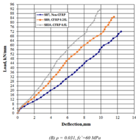
Fig.15. Effect of (CFRP) ratio for HSC Slab Specimens (SN7, SN9 and SN10)
