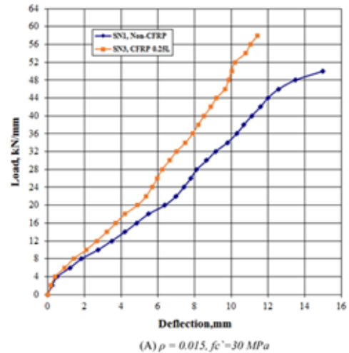
Fig.12. Effect of (CFRP) ratio for NSC Slab Specimens (SN1 and SN3)
