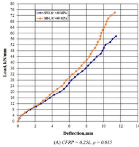
Fig.8. Effect of ( f'_c ) for Strengthened Slab Specimens (SN3 and SN4)
