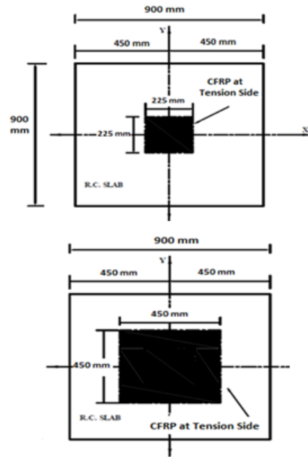
Fig.2. Strengthening with CFRP (0.25L2) and (0.5L2) at tension face
