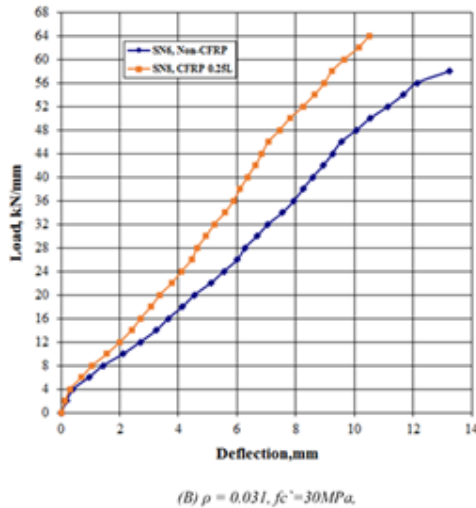
Fig.13. Effect of (CFRP) ratio for NSC Slab Specimens (SN6 and SN8)
