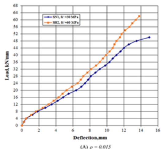
Fig.6. Effect of ( f'_c ) for Non-Strengthened Slab Specimens (SN1 and SN2)
