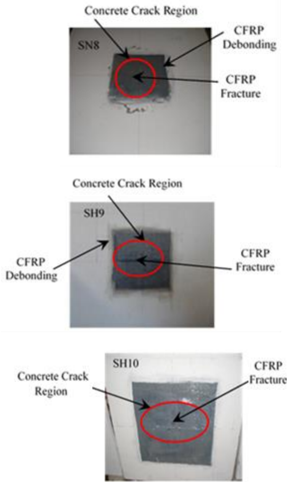
Fig.5. Crack Patterns and Failure Modes of tested slabs
