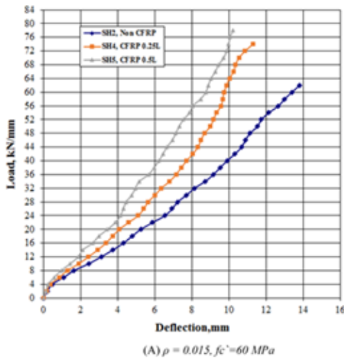
Fig.14. Effect of (CFRP) ratio for HSC Slab Specimens (SN2, SN4 and SN5)
