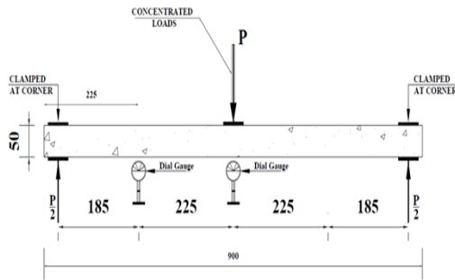
Fig.3. Typical schematic sketch of experimental arrangement and slab specimen setup
