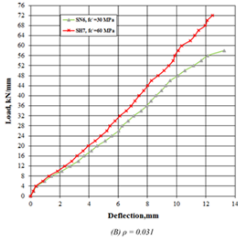
Fig.7. Effect of ( f'_c ) for Non-Strengthened Slab Specimens (SN6 and SN7)
