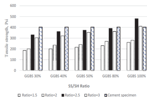
Fig 4. Splitting tensile strength at 28 days for 6 molarity of sodium hydroxide [32]
