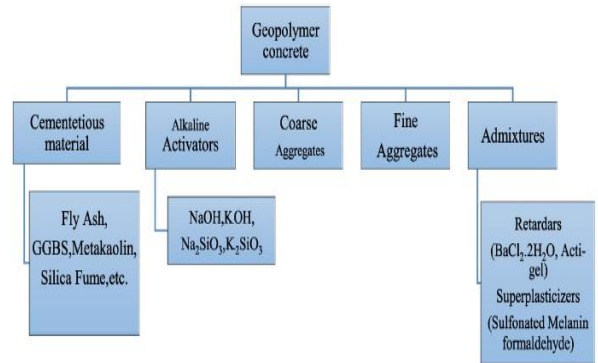
Fig.3.The components of geopolymer concrete[23]
