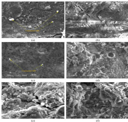
Fig 9. SEM of geopolymer mixtures: (a) P1 at ambient temperature; (b) P1 at 400 °C (c) P3 at ambient temperature; (d) P3 at 400 °C (e) P4 at ambient temperature (f) P4 at 400 °C.[44]
