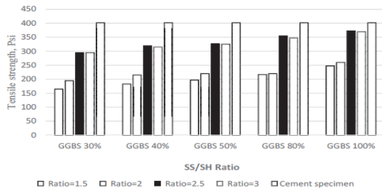
Fig 6. Splitting tensile strength at 28 days for 14 molarity sodium hydroxide[32]
