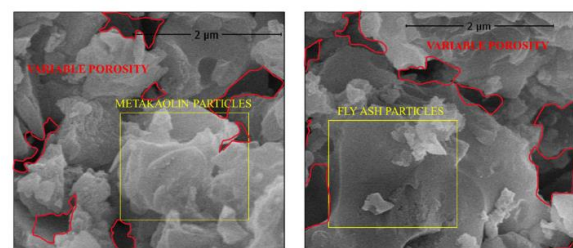
Fig 8. Scanning Electron Microscope picture of fly ash and metakaolin-based Geopolymer Concrete[43]
