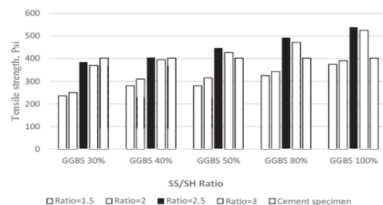
Fig 5. Splitting tensile strength at 28 days for 10 molarity of sodium hydroxide [32]
