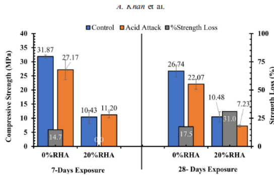
Fig 7 Compressive strength comparison after acid attack on RHA–GP mixtures.[38]
